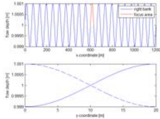
Figure 1: Flow depth before morphodynamic changes start.
