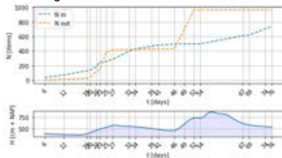
Figure 3: Cumulative representation of fluxes (top) and recorded water level (bottom)
