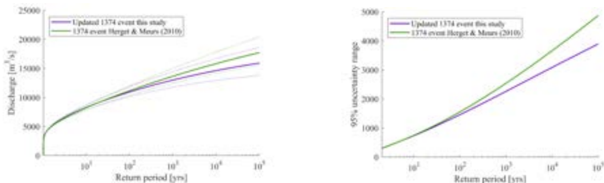
Fig 3. Flood frequency curves and their 95% confidence intervals of data sets corresponding to the reconstructed discharge magnitude of the 1374 flood event of Herget and Meurs's study and this study.
