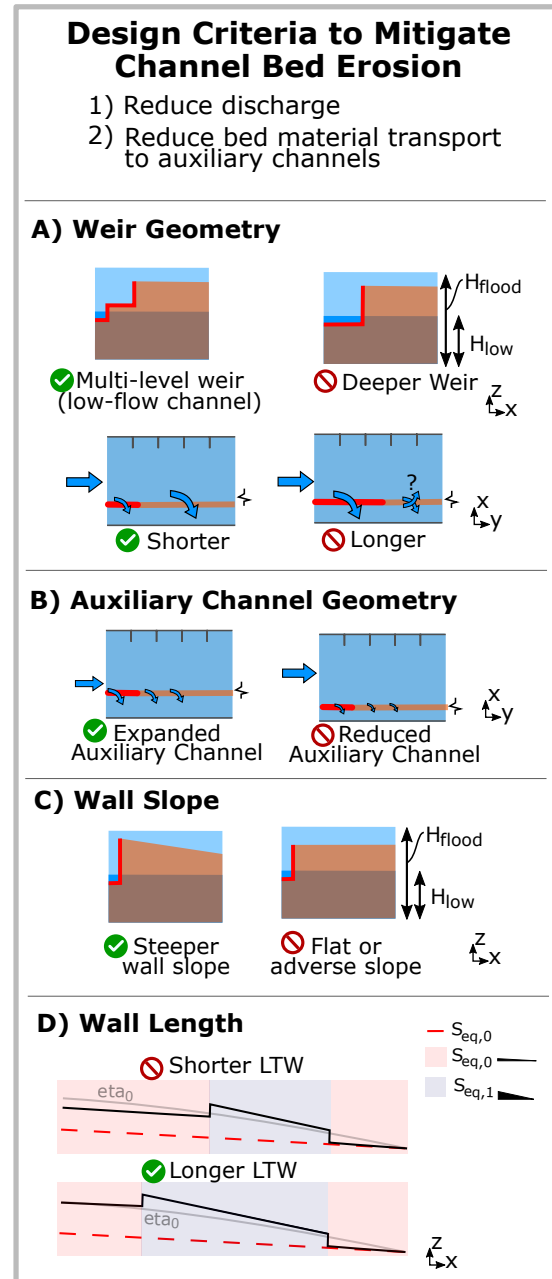
Figure 1: The four main design factors to mitigate erosion with longitudinal training walls.
