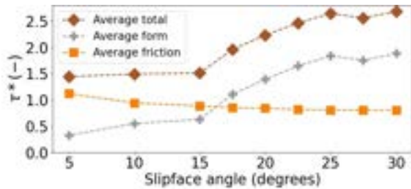
Figure 2: Form, friction and total forces averaged over the three dunes expressed as normalized bed shear stresses for high discharge conditions ( Q = 0.072 \text{ m}^3/\text{s} , S = 3.4 \text{ mm}/\text{m} ).
