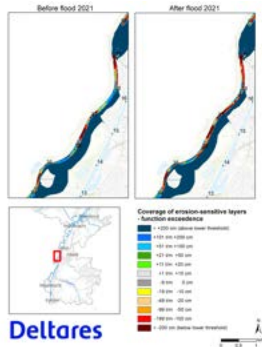
Figure 2: The function exceedence for the function cover on top of erosion-sensitive layers before and after the summer flood of 2021.
