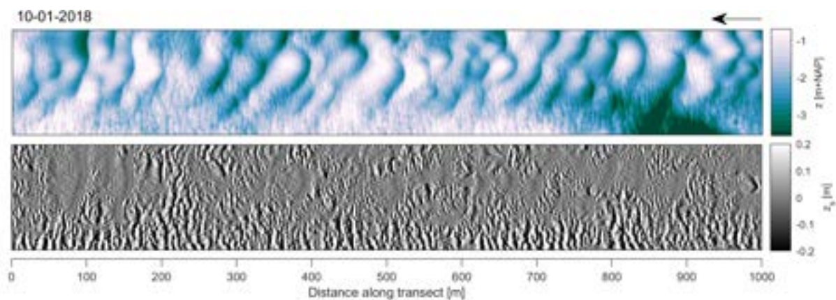
Figure 1: A bathymetric map before and after decomposition. The first panel shows the initial bathymetry. The second panel shows the secondary bedforms.
