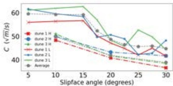
Figure 3: Calculated Chézy values for different slipface angles. Data are from high (H: Q = 0.072 \text{ m}^3/\text{s} , S = 3.4 \text{ mm}/\text{m} ) and low (L: Q = 0.130 \text{ m}^3/\text{s} , S = 1.0 \text{ mm}/\text{m} ) discharge conditions for dunes 1, 2, and 3. The included average is the average per condition.
