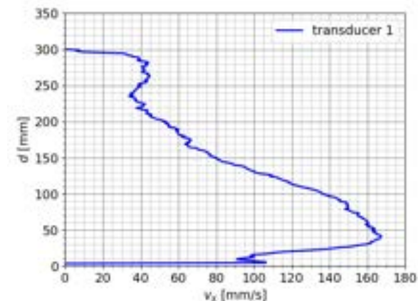
Figure 3. Mean velocity profile at position B (Figure 1). The velocities were averaged from t \sim 7 s (snapshot B, Figure 1) to t \sim 23 s (snapshot E, Figure 1) from the start of the experiment.
