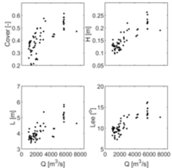
Figure 3: The fraction of the river bed covered with secondary bedforms and secondary bedform properties (height, H , length, L , and the max. lee side slope) for different discharge levels. The presented data is based on analysis of bed elevation scans at km 35 in the river Waal, near Tiel.
